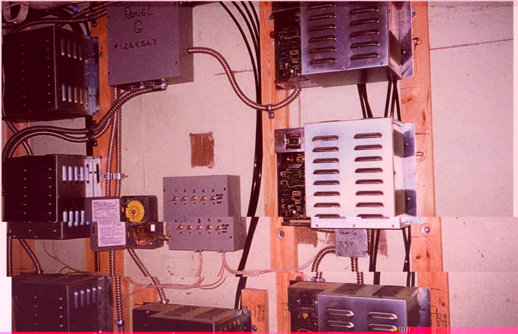
▲ Control boxes in Leadville, CO - ten zones with programmable timer control ▲
